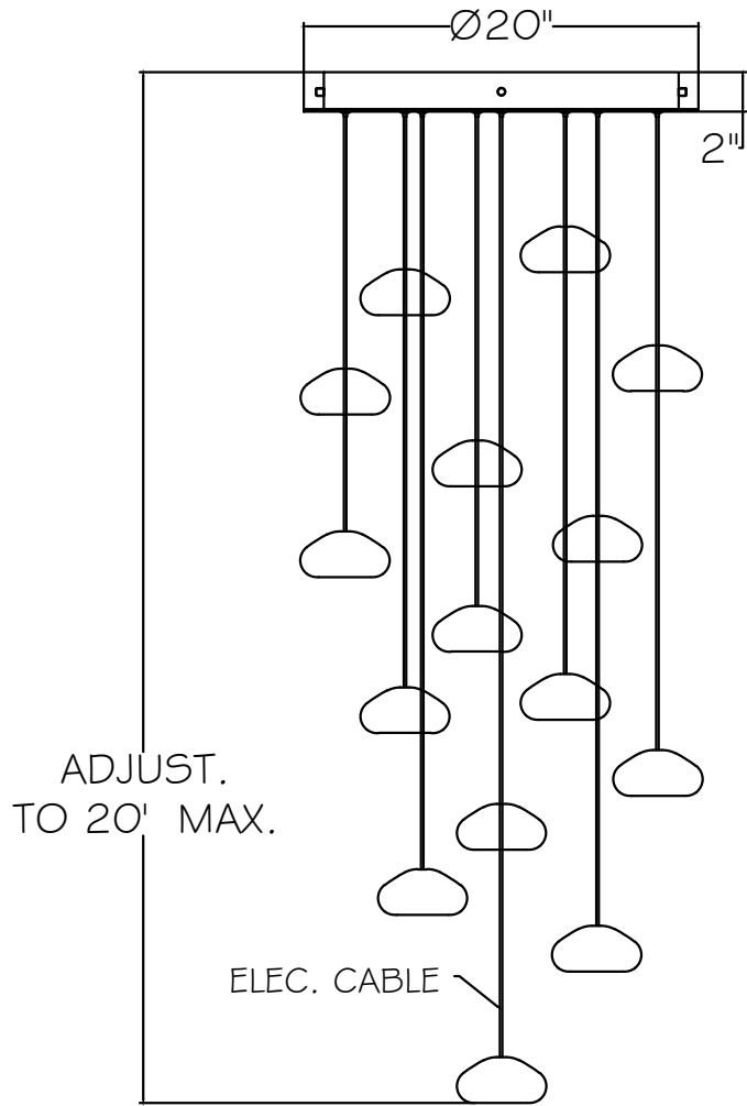
FRONT VIEW
