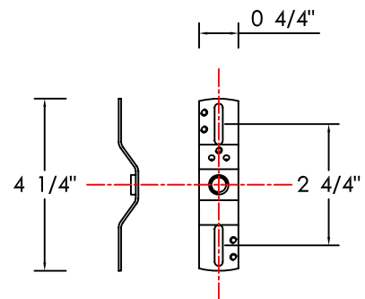
Mounting Strap Dimensions
