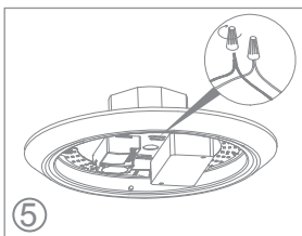
Wire connection.
